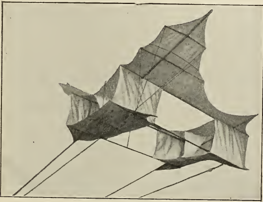
FIG. 72.—Cody's kite.
