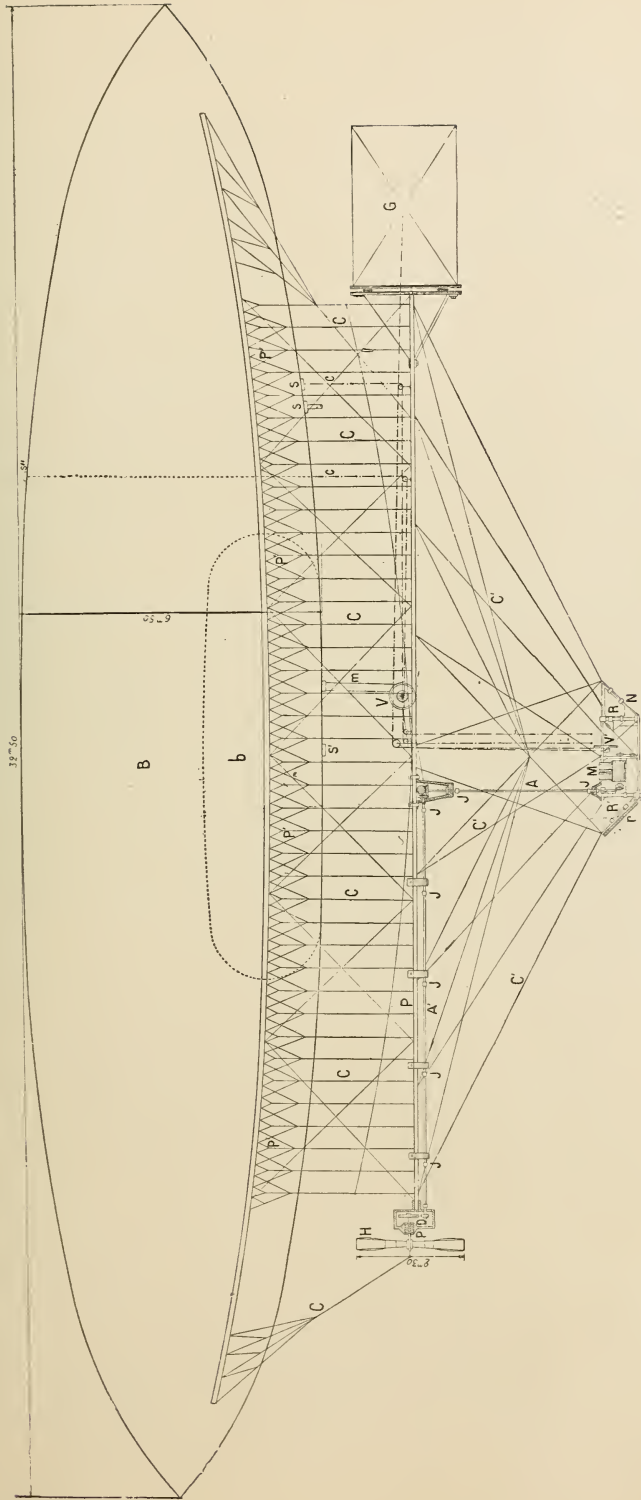
FIG. 45.—Count de la Vaux's dirigible balloon.
