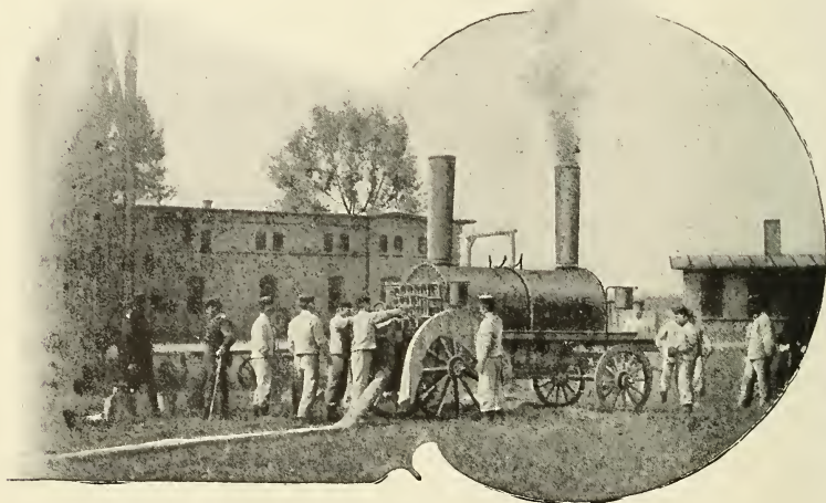
FIG. 88.—Steam winch for pulling in a captive balloon.
