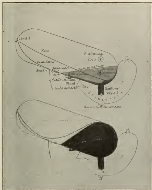
Fig. 116.—Drawing showing the design of the kite-balloon.
