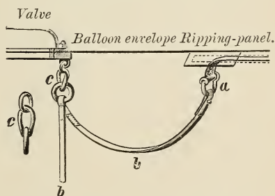
FIG. 112.—Arrangements for ripping-panel.
