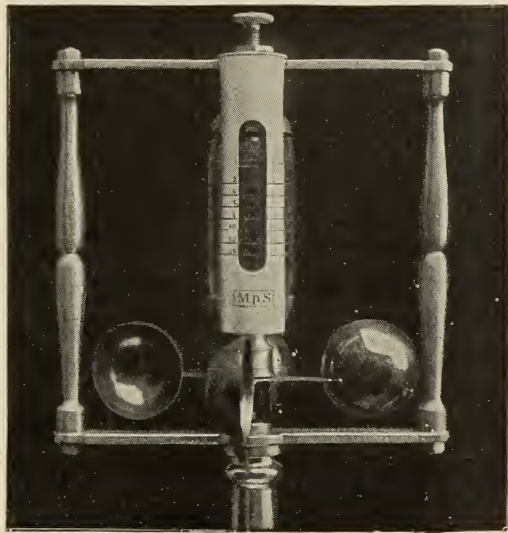
FIG. 37.—Gradenwitz anemometer.
