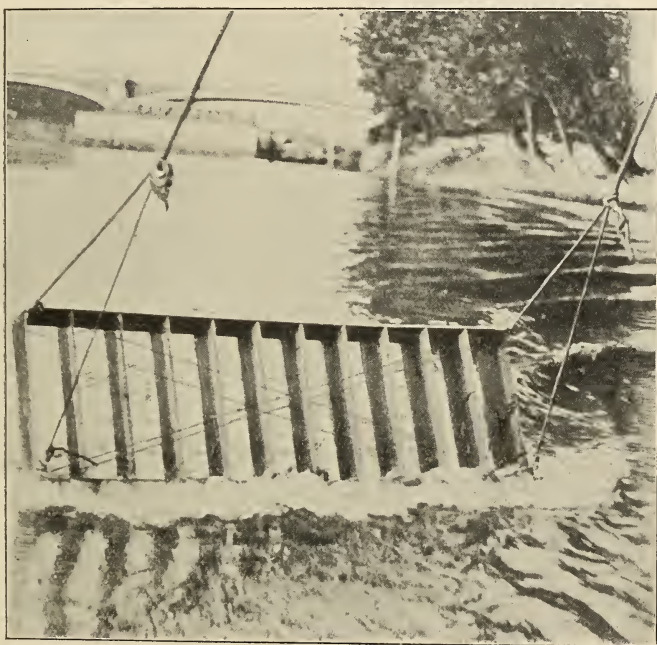
FIG. 133.—Count de la Vault's deviator in action.
