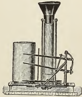
FIG. 171.—Baro-thermo-hygrograph, designed for recording balloons by Dr. Hergesell, and made by Bosch, of Strassburg.
