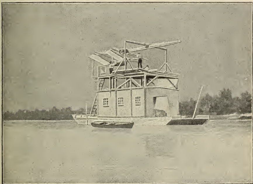
FIG. 56.—Starting arrangements for Professor Langley's flying machine.
